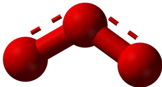
Ball-and-stick model of the O_3 molecule
