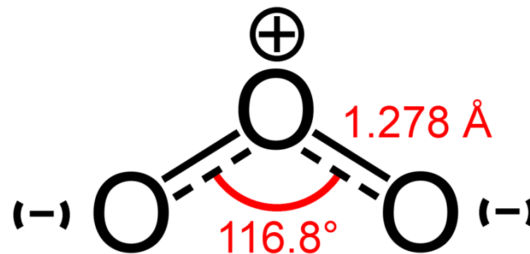
Ozone 1,3-dipole moment
